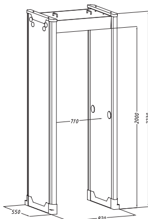
Side information
